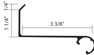
3 - 3/8" Female Hinge
